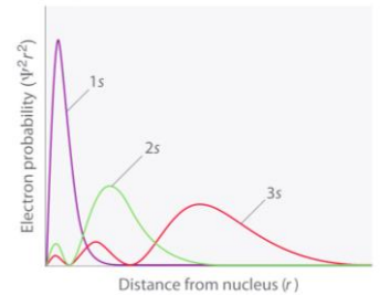
(c) Radial probability
